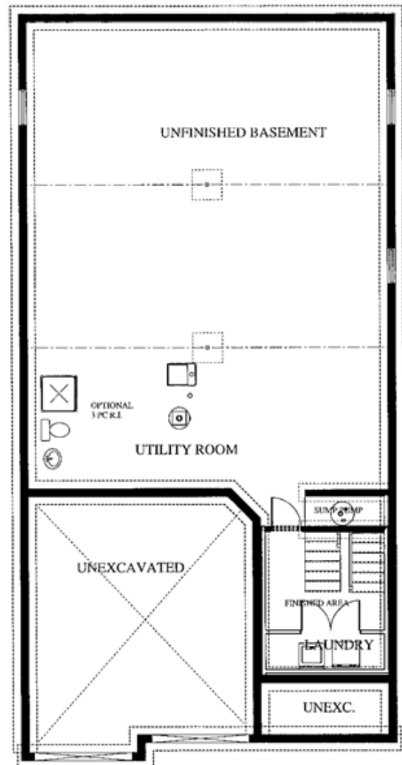
FOUNDATION PLAN
