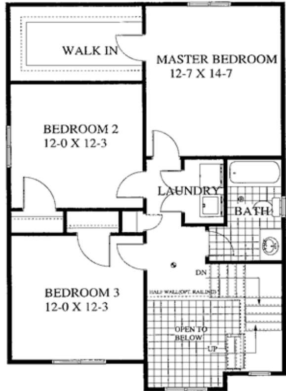
SECOND FLOOR PLAN 937 SQFT
