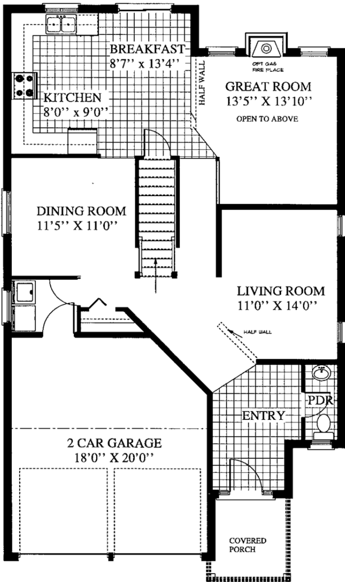
MAIN FLOOR PLAN 1100 SQFT
