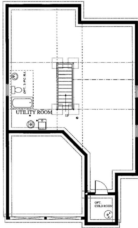
FOUNDATION PLAN
