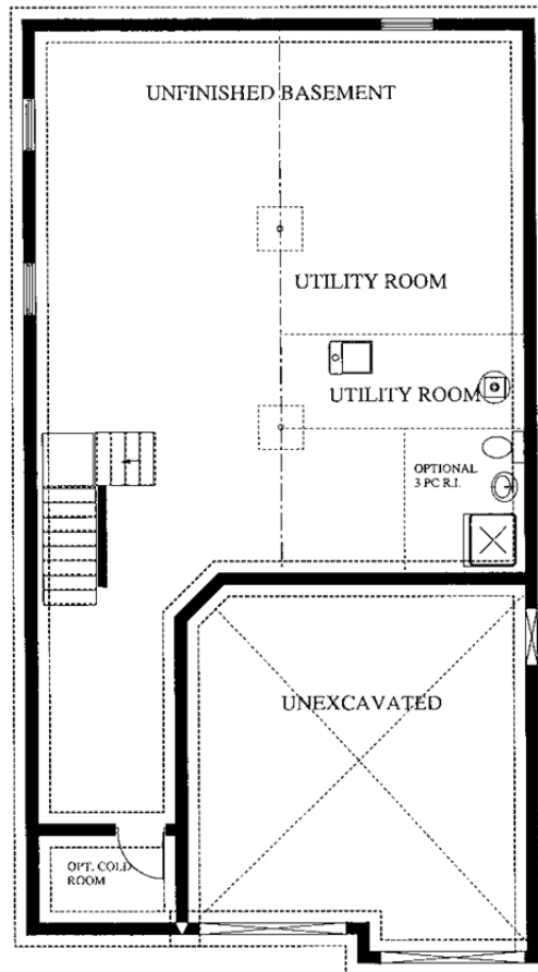
FOUNDATION PLAN
