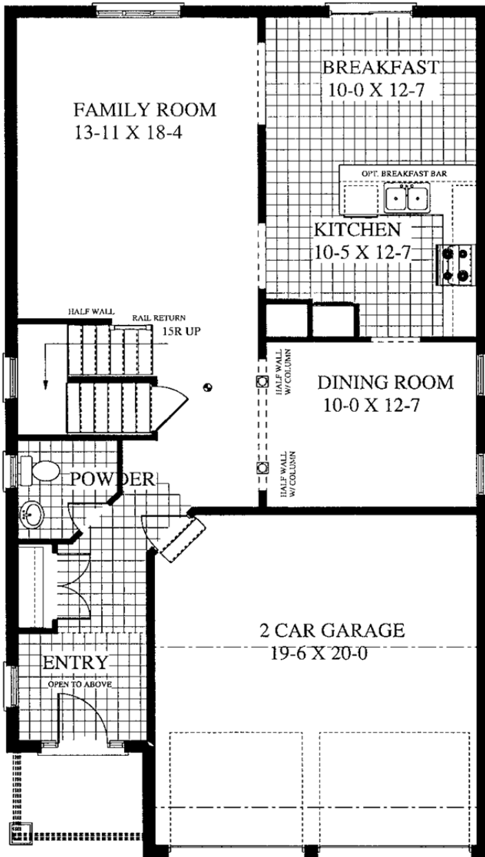
MAIN FLOOR PLAN 1024 SQFT
