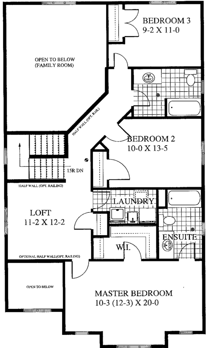
SECOND FLOOR PLAN B 1404 SQFT
