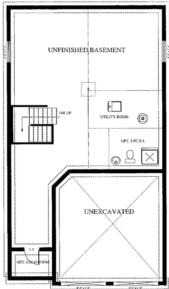
FOUNDATION PLAN
