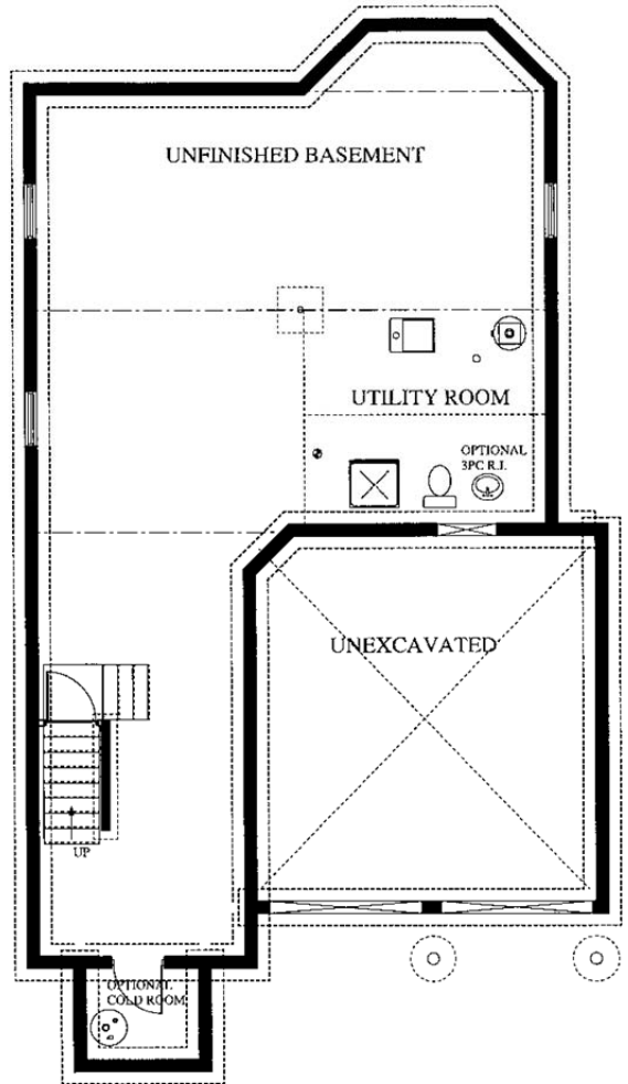
FOUNDATION PLAN
