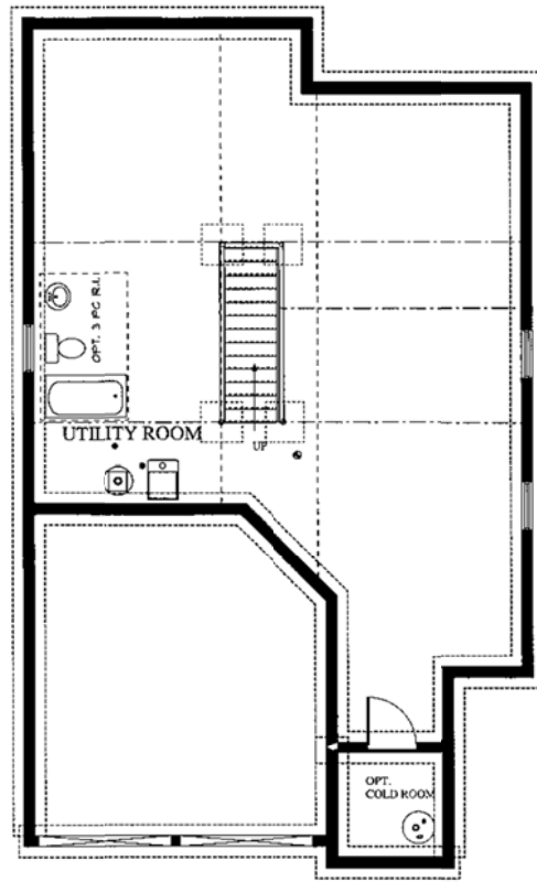
FOUNDATION PLAN
