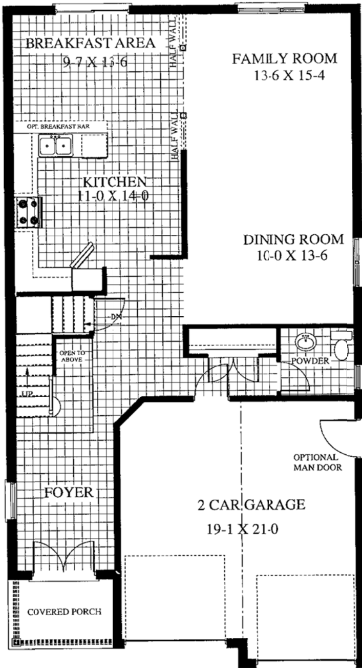
MAIN FLOOR PLAN 1075 SQFT
