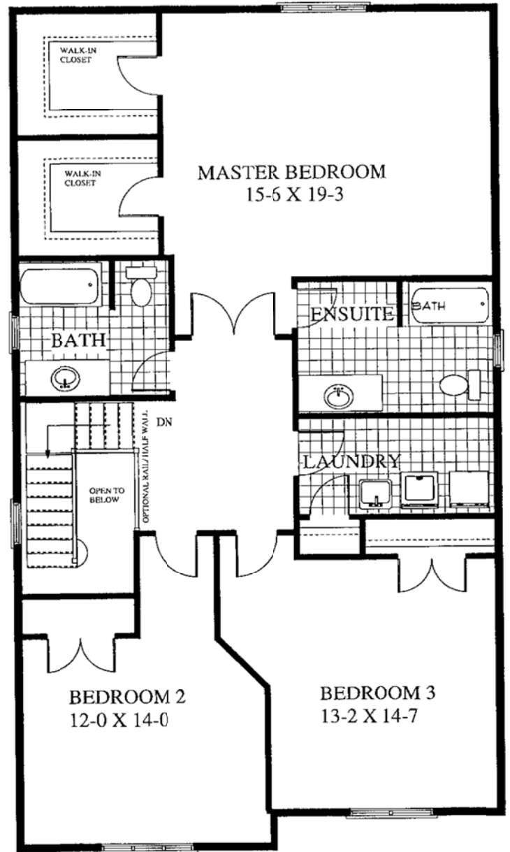
SECOND FLOOR PLAN 1435 SQFT
