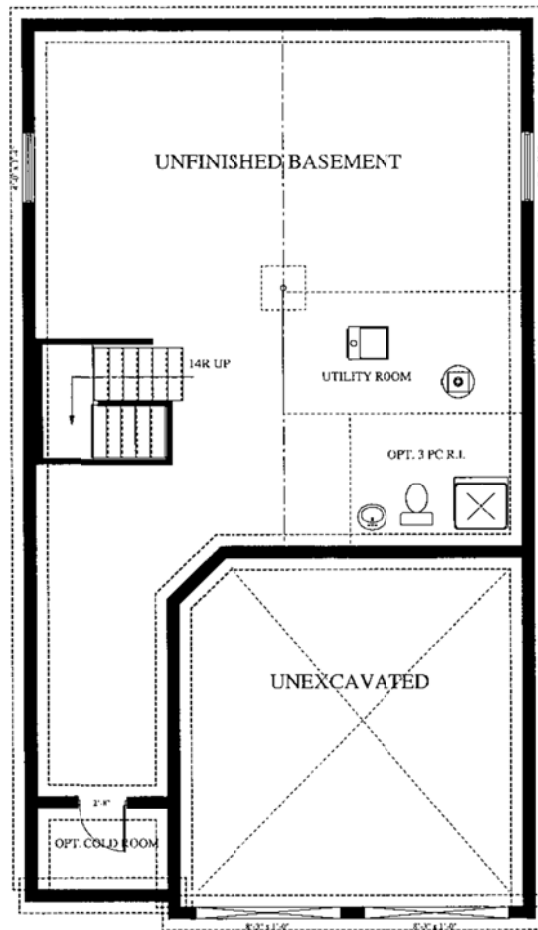
FOUNDATION PLAN
