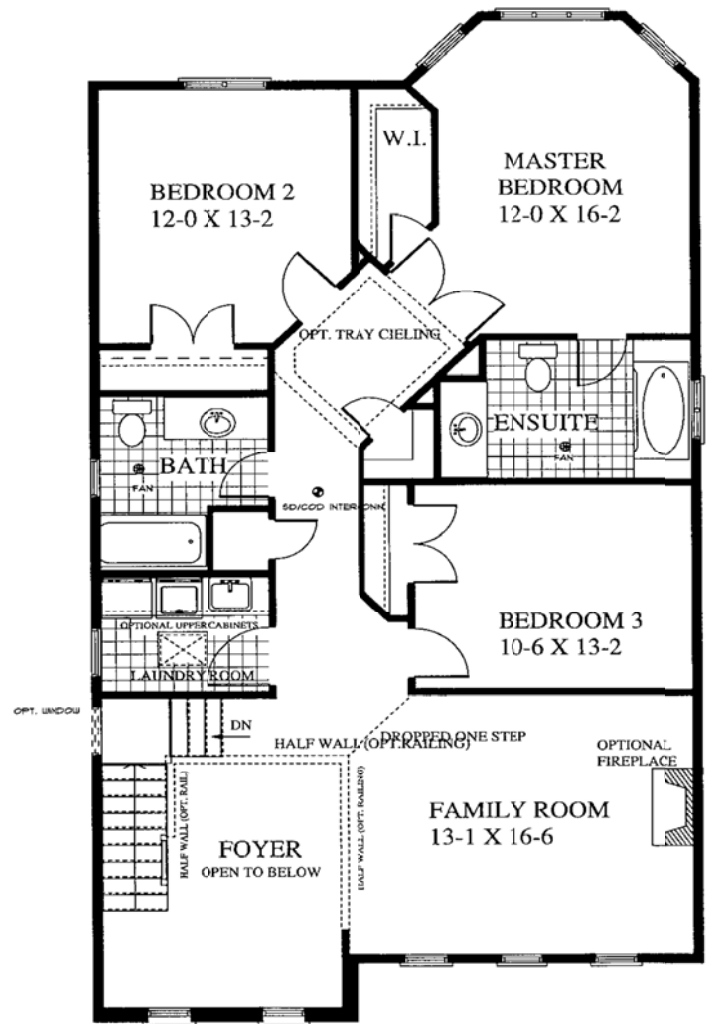
SECOND FLOOR PLAN 1397 SQFT
