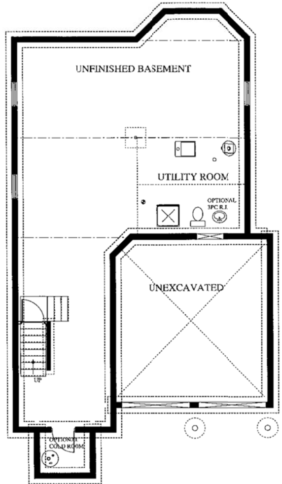
FOUNDATION PLAN
