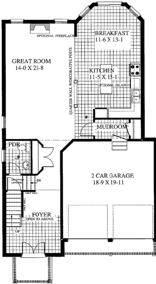
MAIN FLOOR PLAN 1049 SQFT
